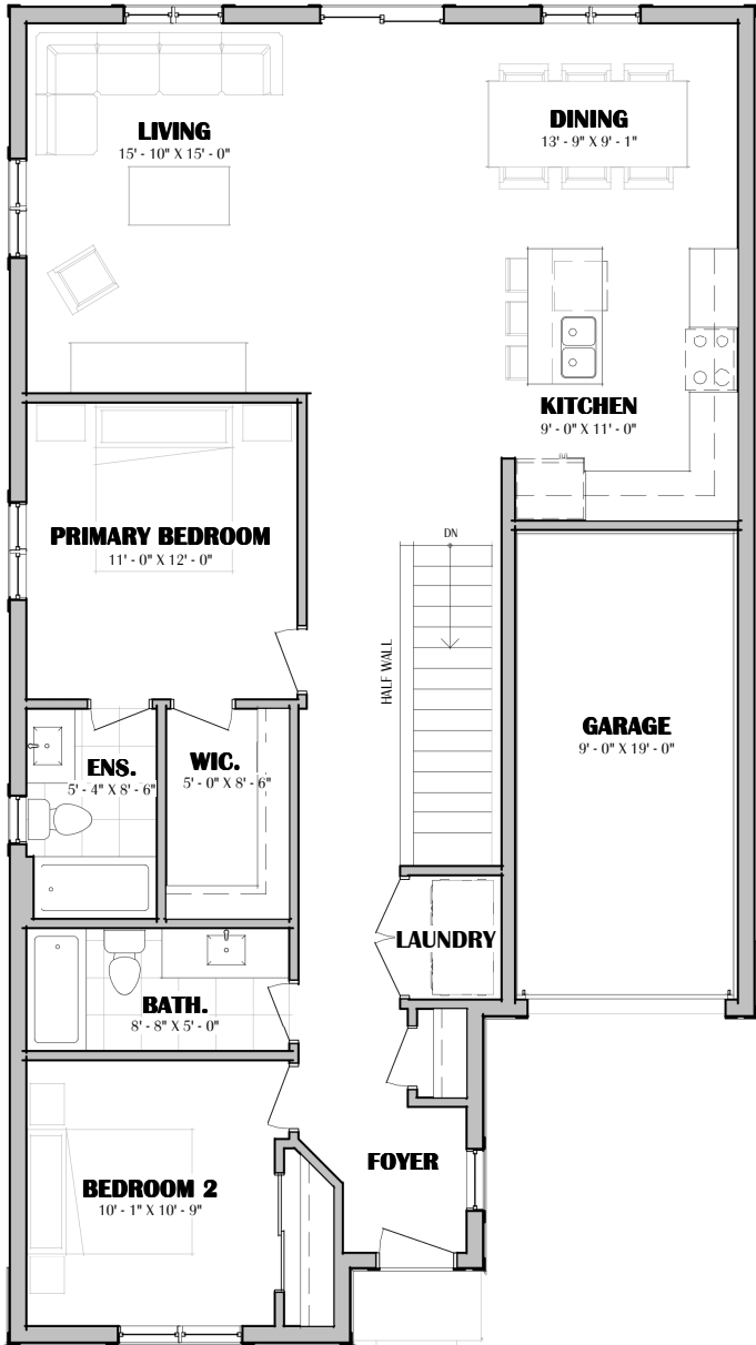
1ST FLOOR
